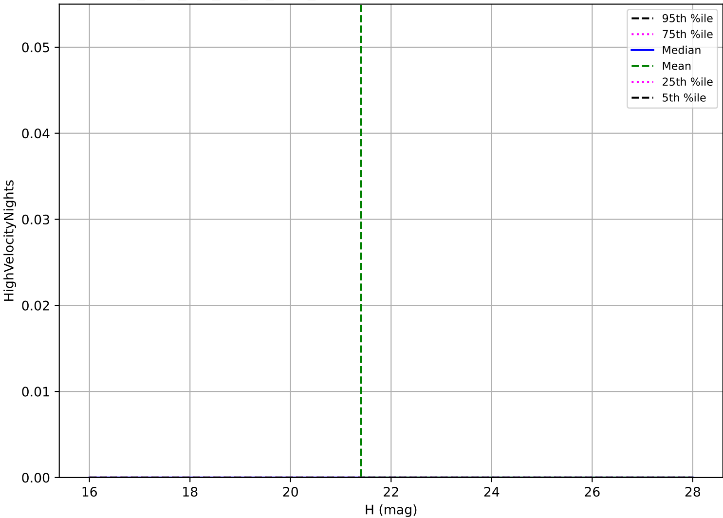
too_elab_r32_d2_gz_v3.4_10yrs: Vatira High velocity pair detection loss
