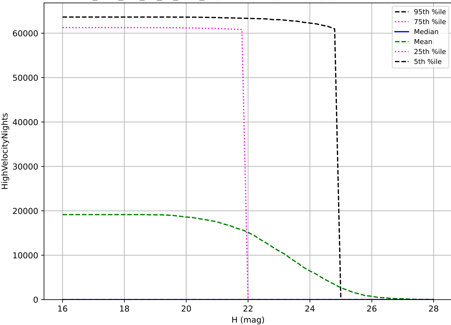
too_elab_r32_d2_gz_v3.4_10yrs: NEO High velocity pair detection loss
