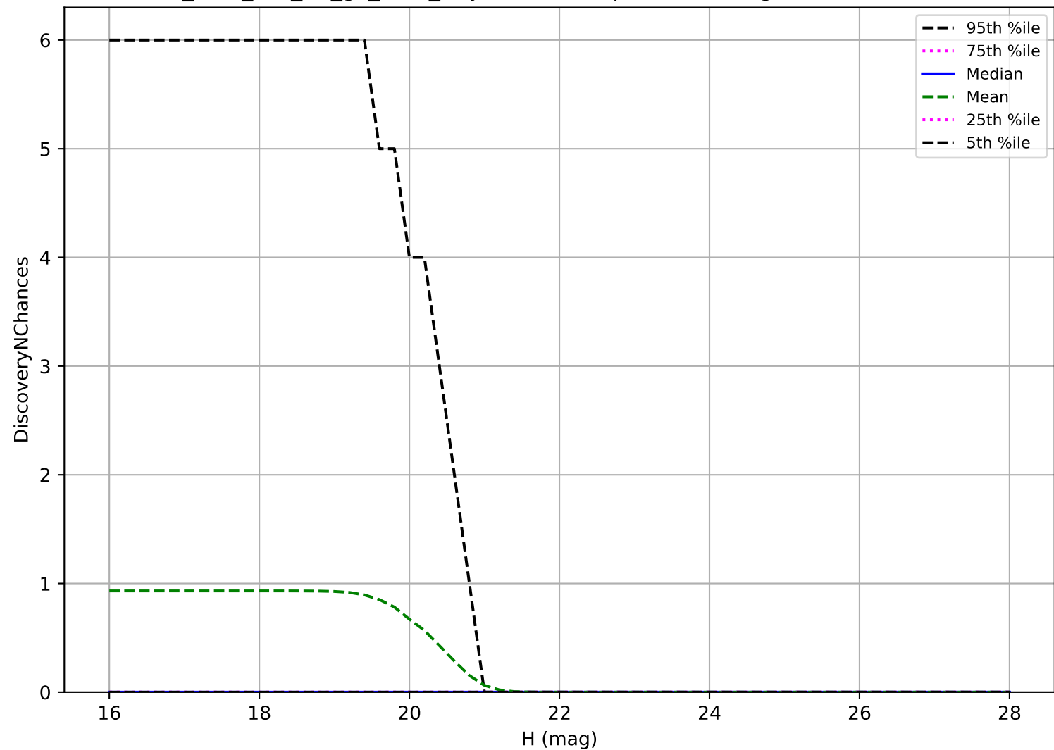
too_elab_r32_d2_gz_v3.4_10yrs: Vatira 3 pairs in 15 nights detection loss
