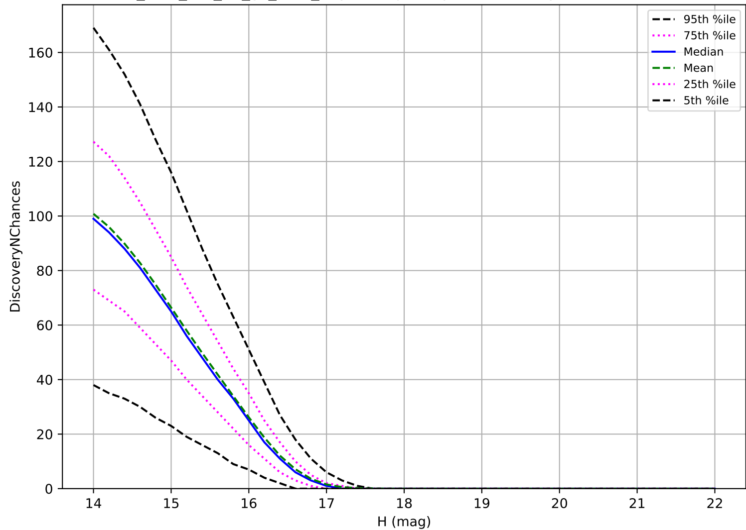
too_elab_r32_d2_gz_v3.4_10yrs: Trojan 3 pairs in 15 nights detection loss
