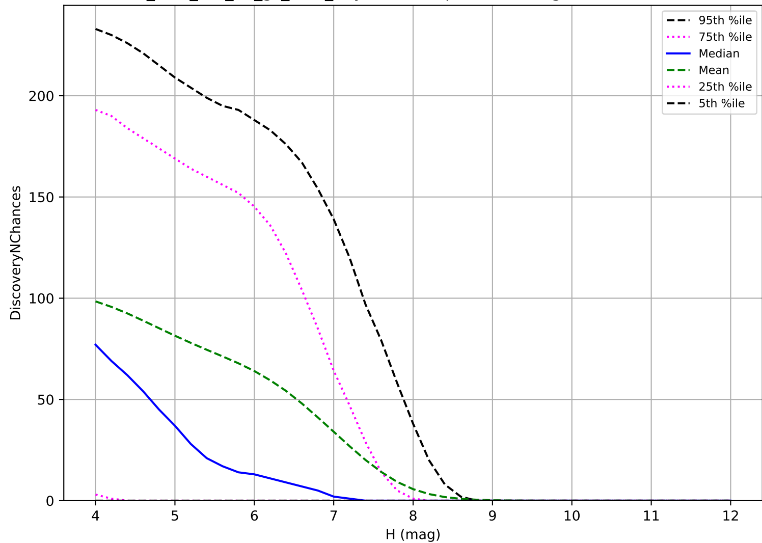
too_elab_r32_d2_gz_v3.4_10yrs: TNO 3 pairs in 15 nights detection loss
