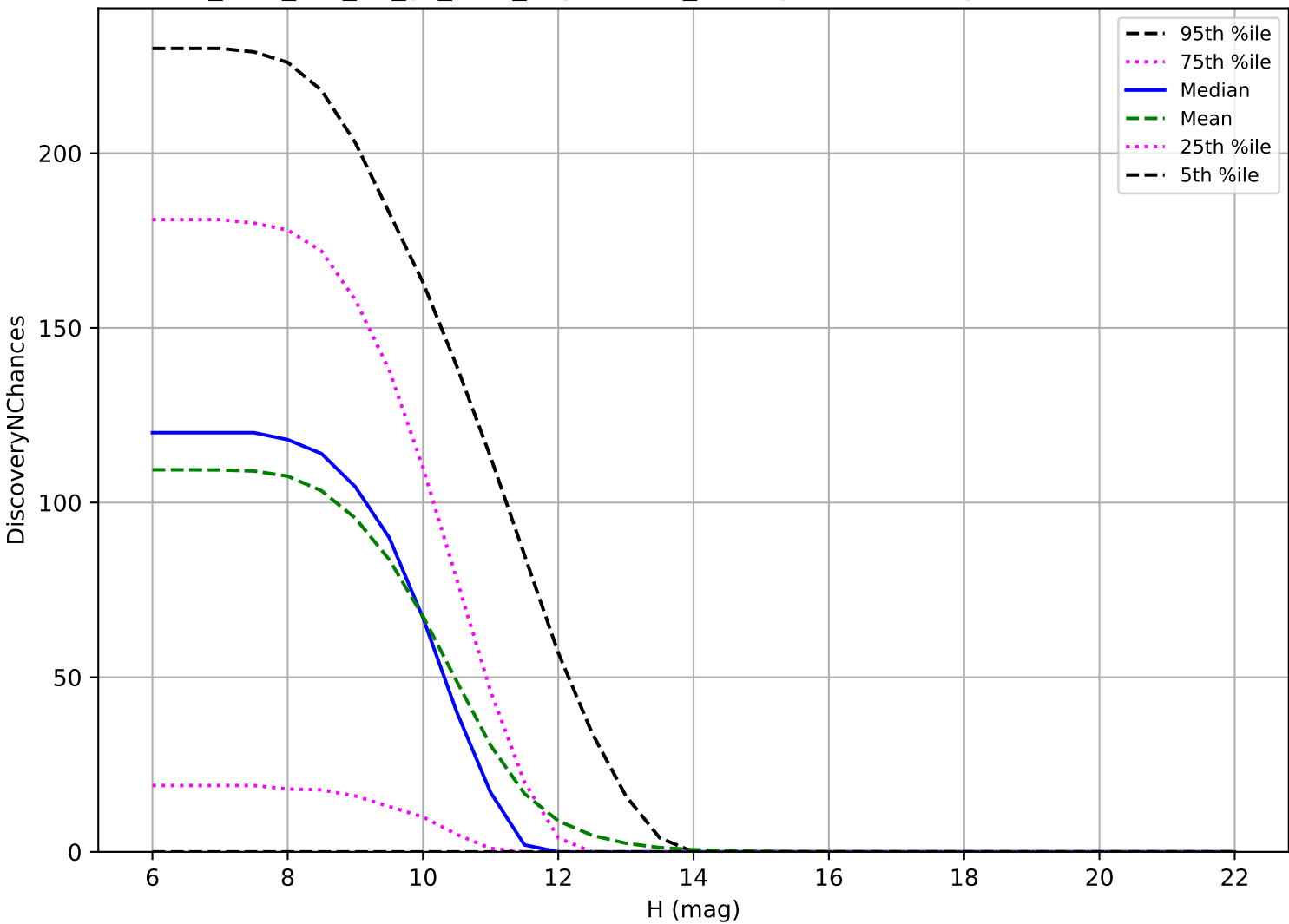
too_elab_r32_d2_gz_v3.4_10yrs: OCC_r20 3 pairs in 15 nights detection loss
