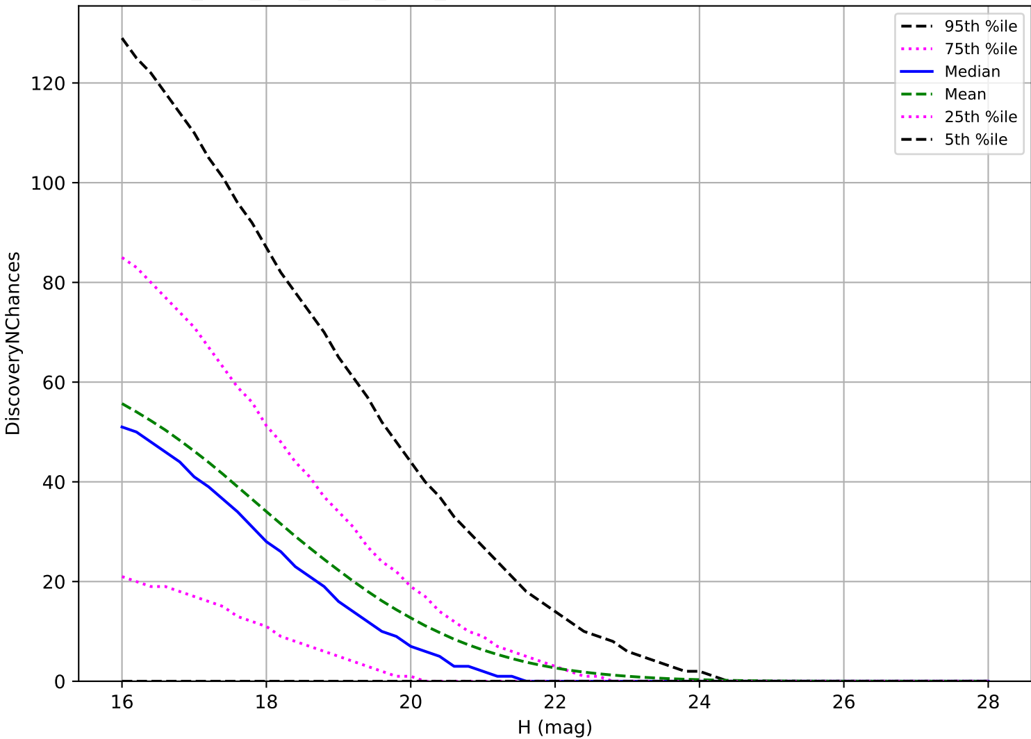
too_elab_r32_d2_gz_v3.4_10yrs: NEO 3 pairs in 15 nights detection loss
