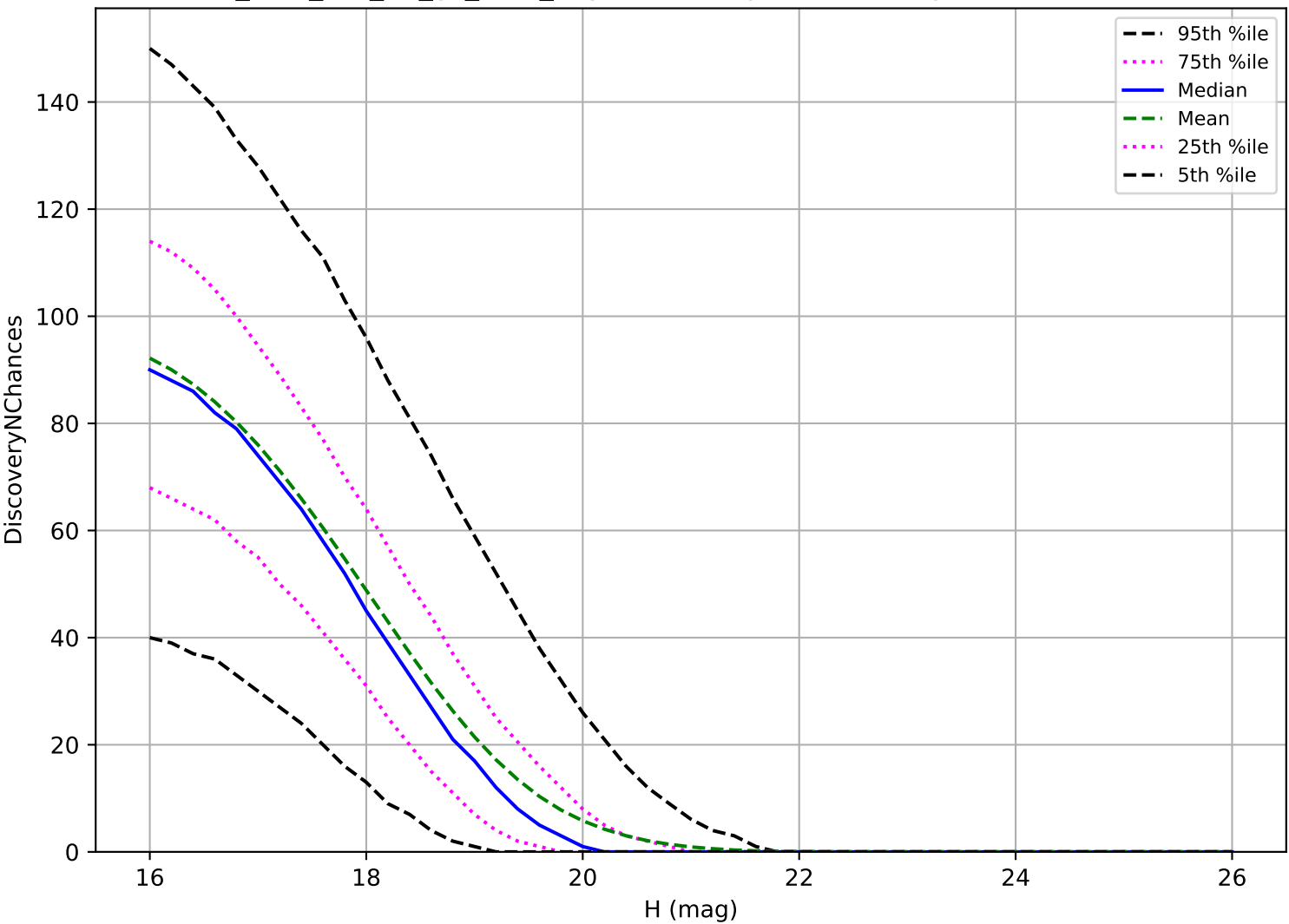
too_elab_r32_d2_gz_v3.4_10yrs: MBA 3 pairs in 15 nights detection loss
