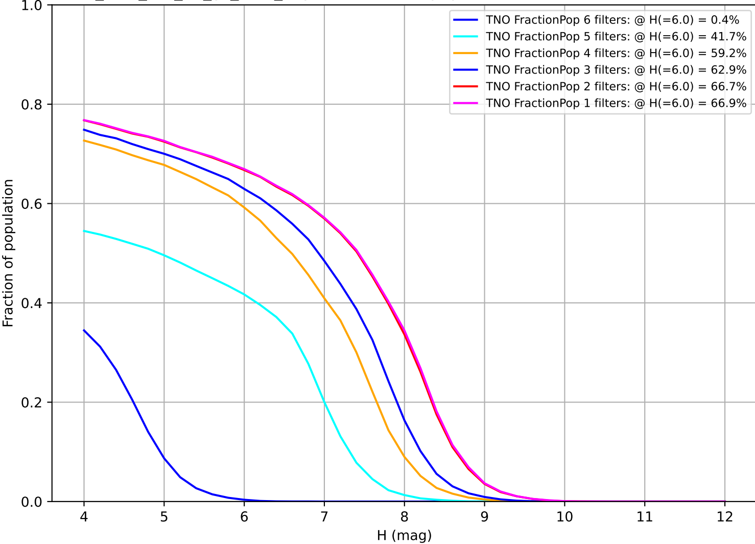
too_elab_r32_d2_gz_v3.4_10yrs: Fraction of population with colors in X filters TNO
