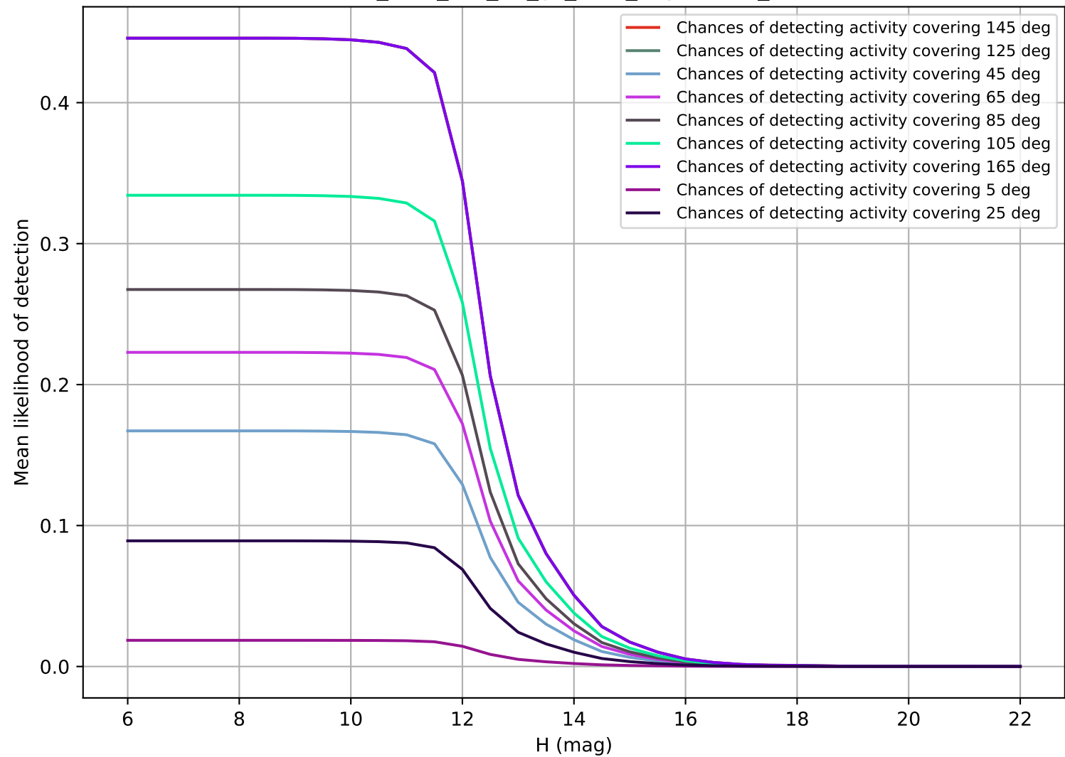
too_elab_r32_d2_gz_v3.4_10yrs OCC_r20
