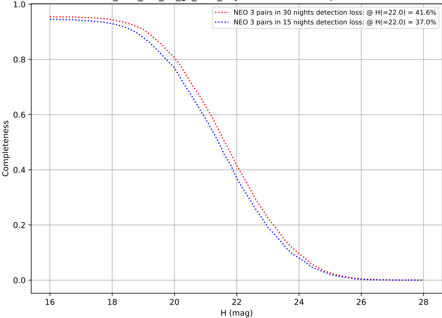
too_elab_r32_d2_gz_v3.4_10yrs: DifferentialCompleteness
