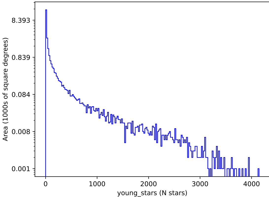
too_elab_r32_d2_gz_v3.4_10yrs : young_stars
