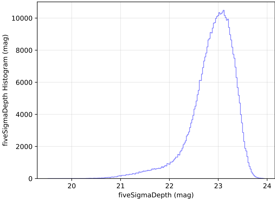
too_elab_r32_d2_gz_v3.4_10yrs z: fiveSigmaDepth Histogram
