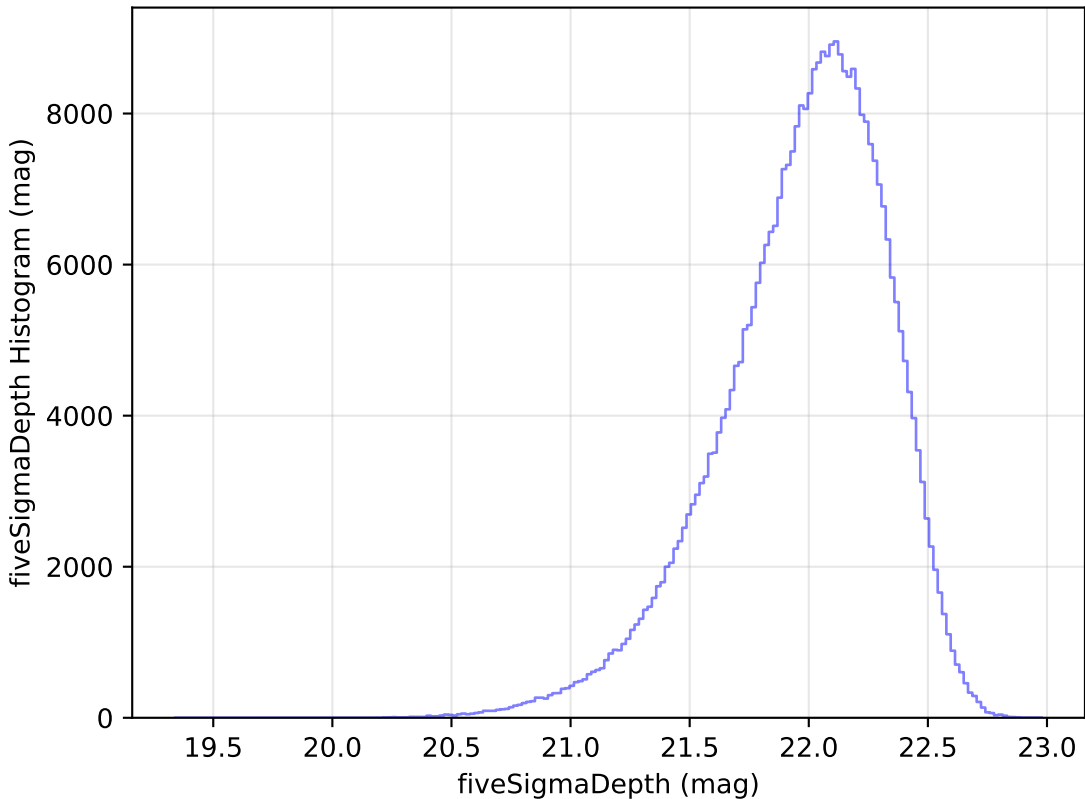
too_elab_r32_d2_gz_v3.4_10yrs y: fiveSigmaDepth Histogram
