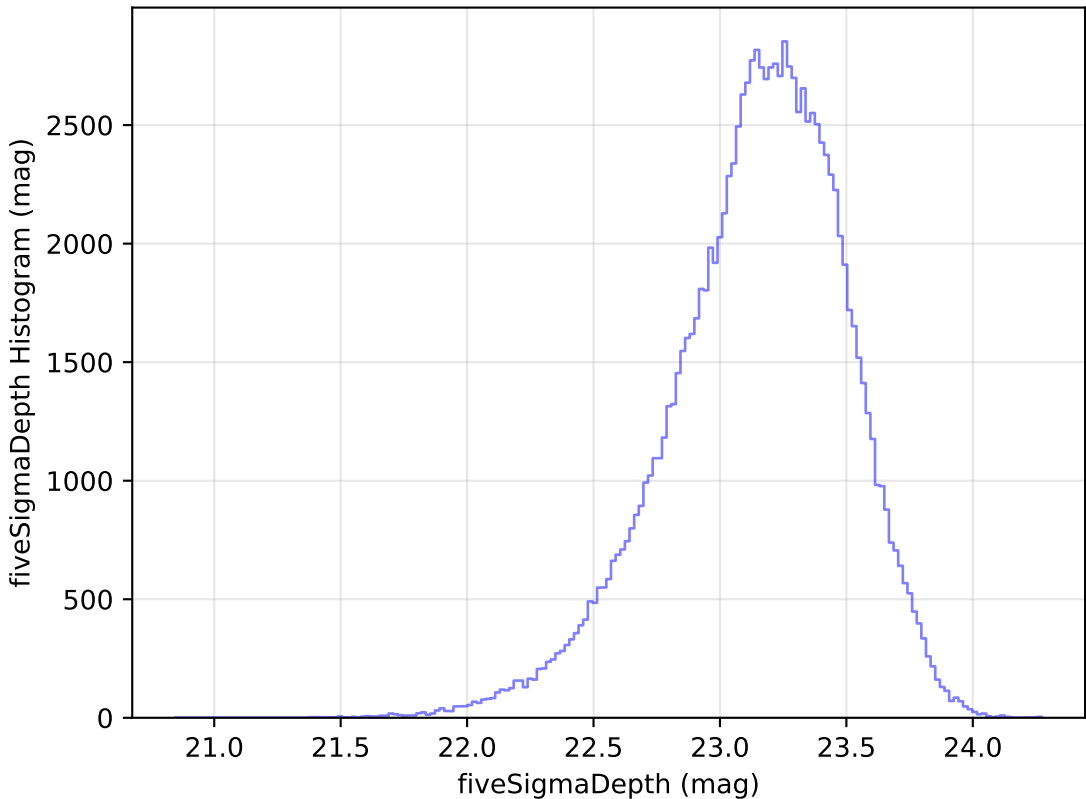
too_elab_r32_d2_gz_v3.4_10yrs u: fiveSigmaDepth Histogram
