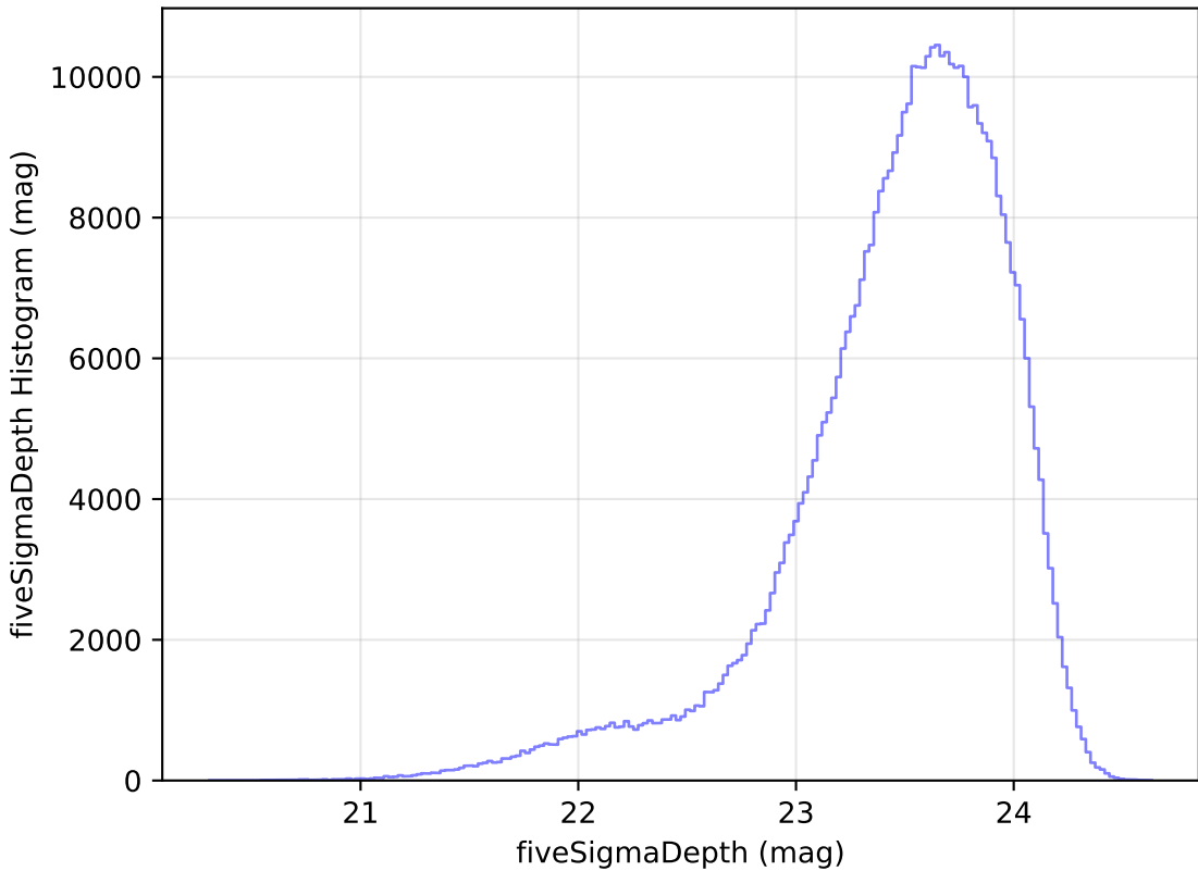
too_elab_r32_d2_gz_v3.4_10yrs i: fiveSigmaDepth Histogram
