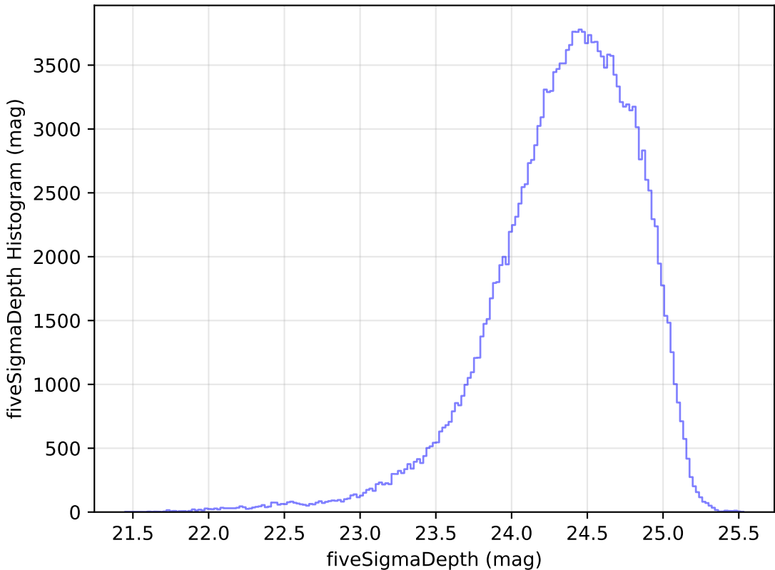
too_elab_r32_d2_gz_v3.4_10yrs g: fiveSigmaDepth Histogram
