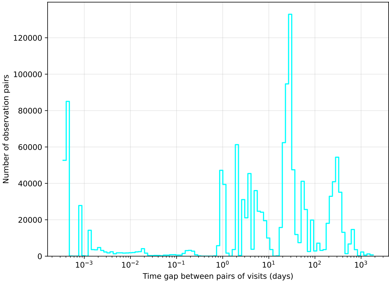
too_elab_r32_d2_gz_v3.4_10yrs u band: Tgaps observationStartMJD
