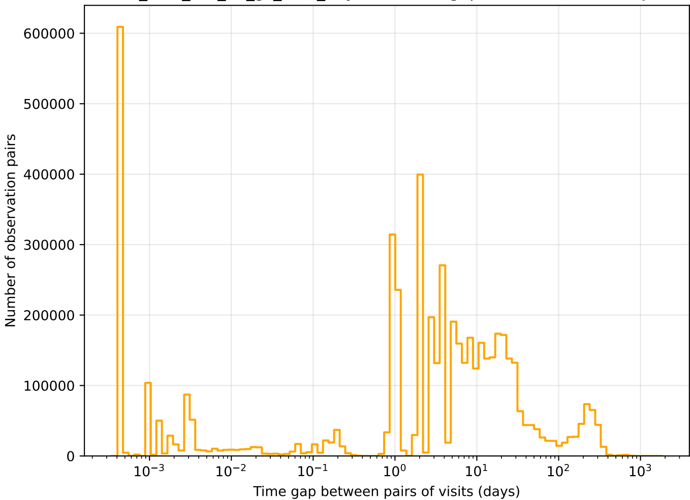
too_elab_r32_d2_gz_v3.4_10yrs r band: Tgaps observationStartMJD
