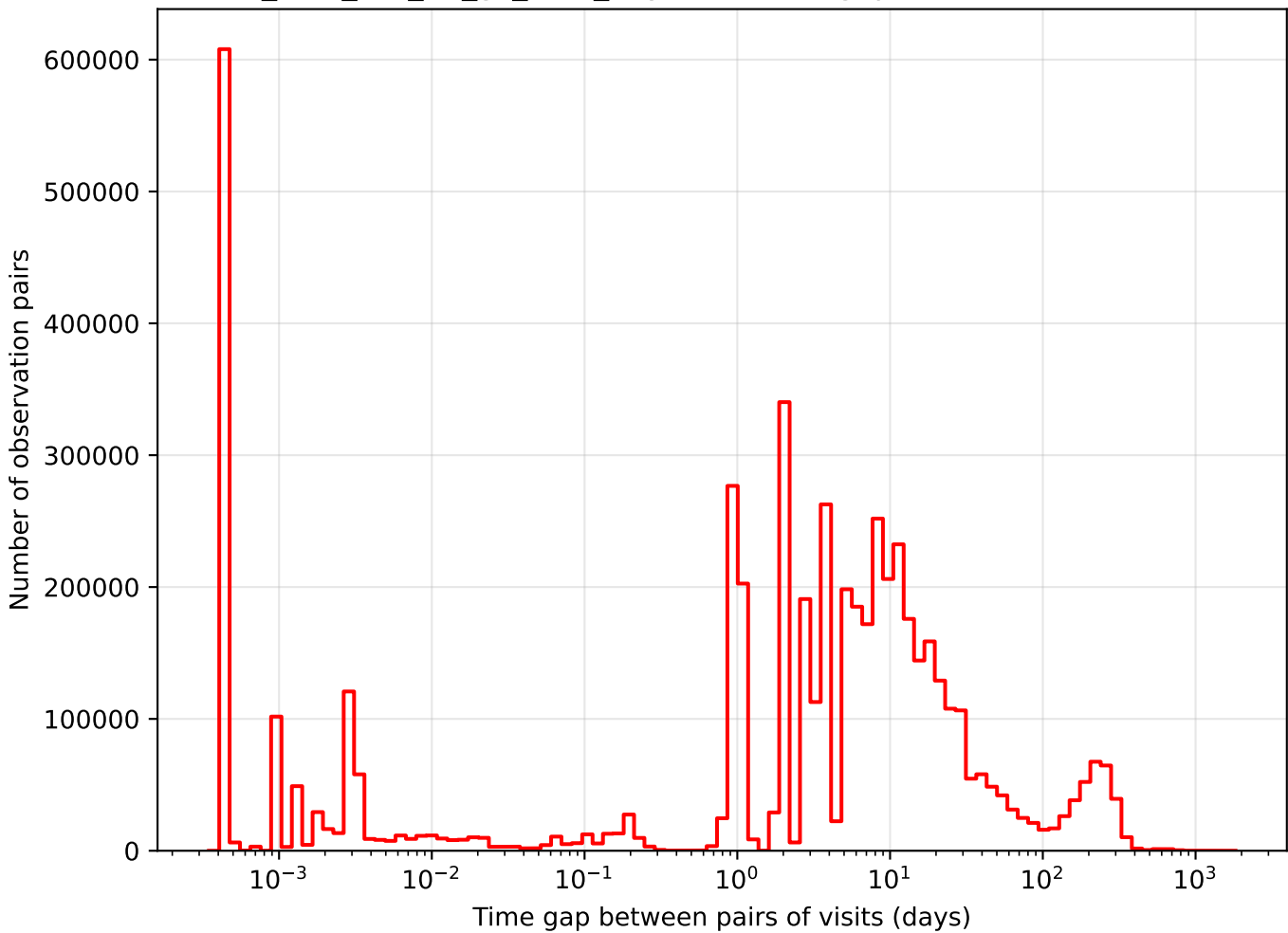
too_elab_r32_d2_gz_v3.4_10yrs i band: Tgaps observationStartMJD
