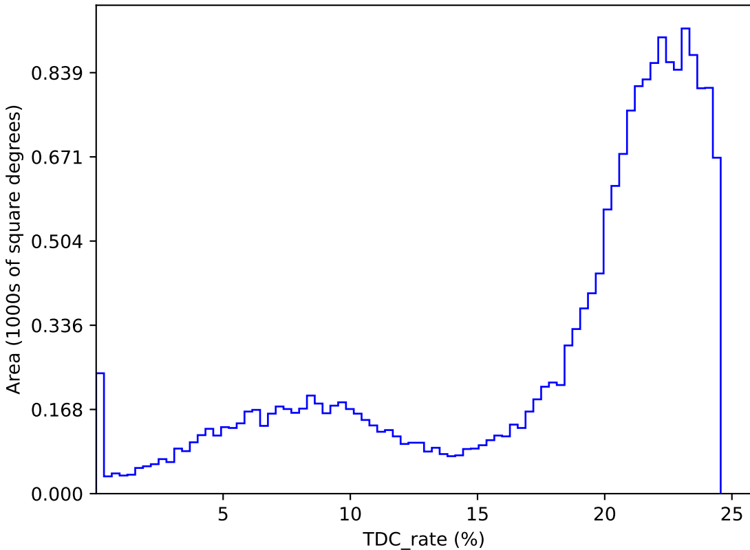
too_elab_r32_d2_gz_v3.4_10yrs : TDC_rate
