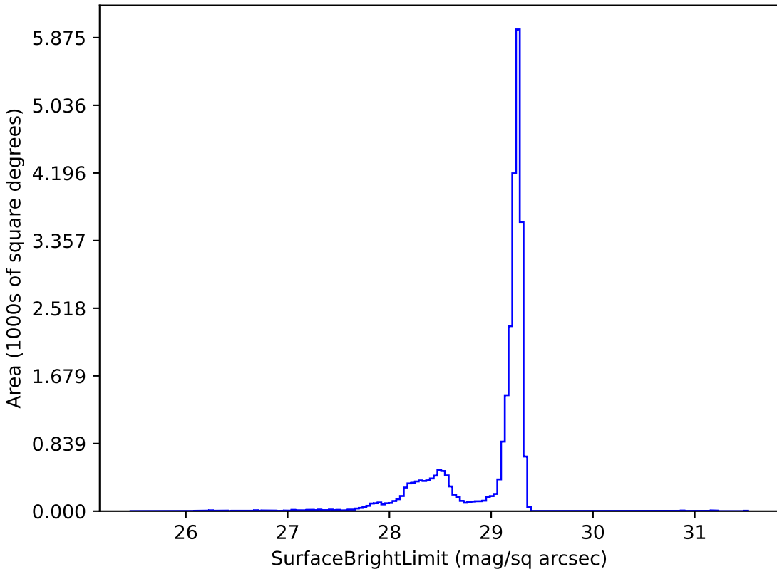
too_elab_r32_d2_gz_v3.4_10yrs z: SurfaceBrightLimit
