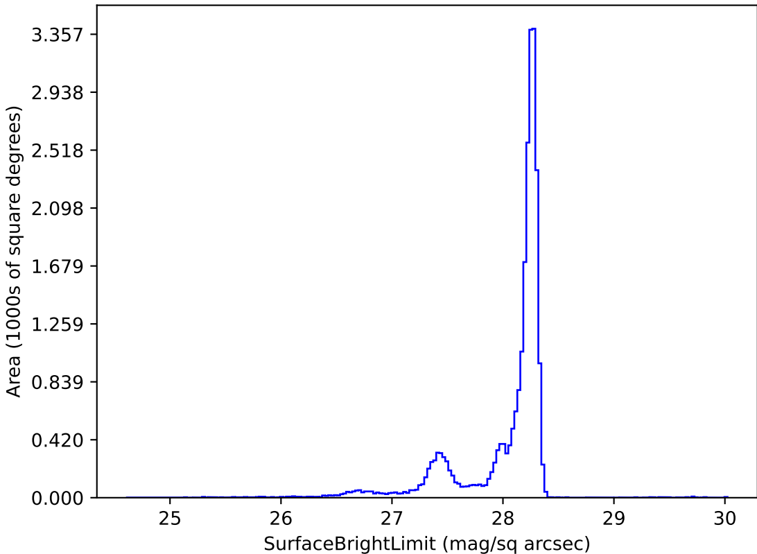
too_elab_r32_d2_gz_v3.4_10yrs y: SurfaceBrightLimit
