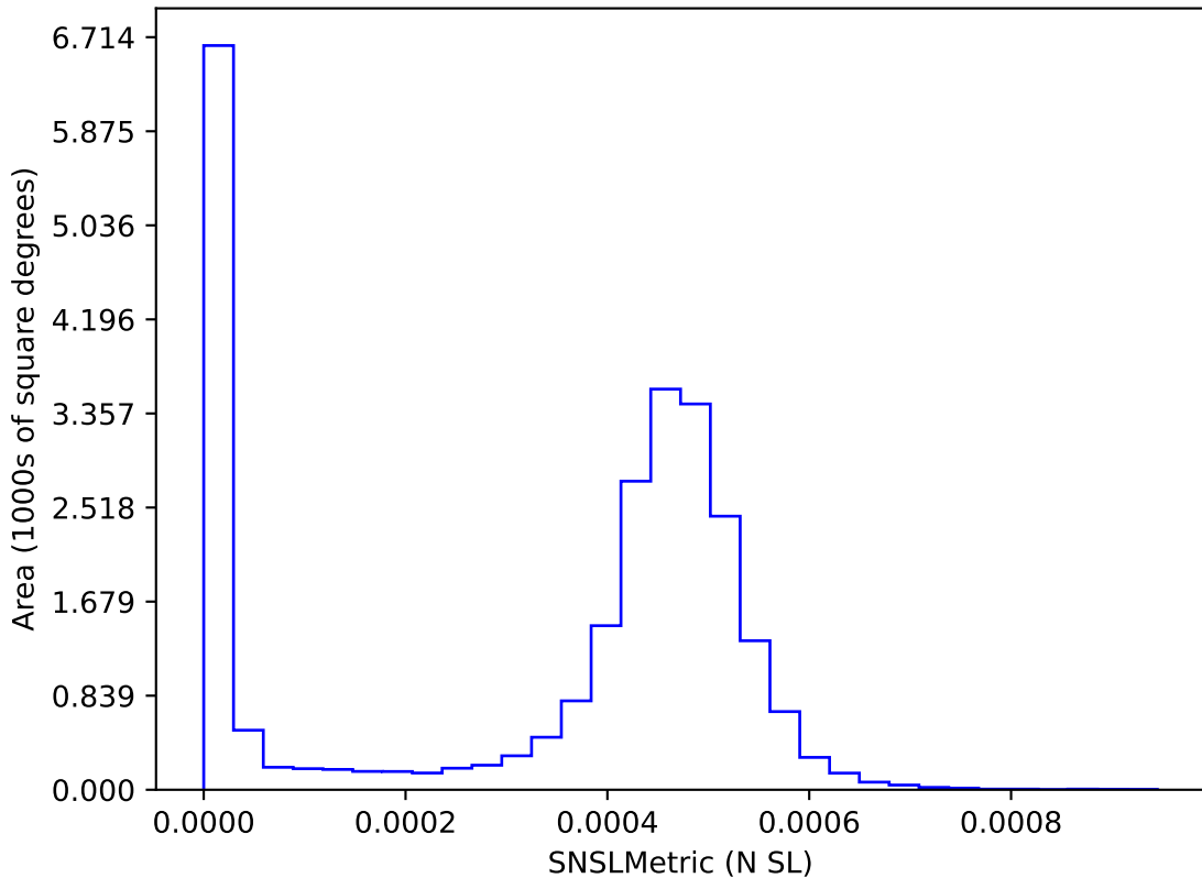
too_elab_r32_d2_gz_v3.4_10yrs : SNSLMetric
