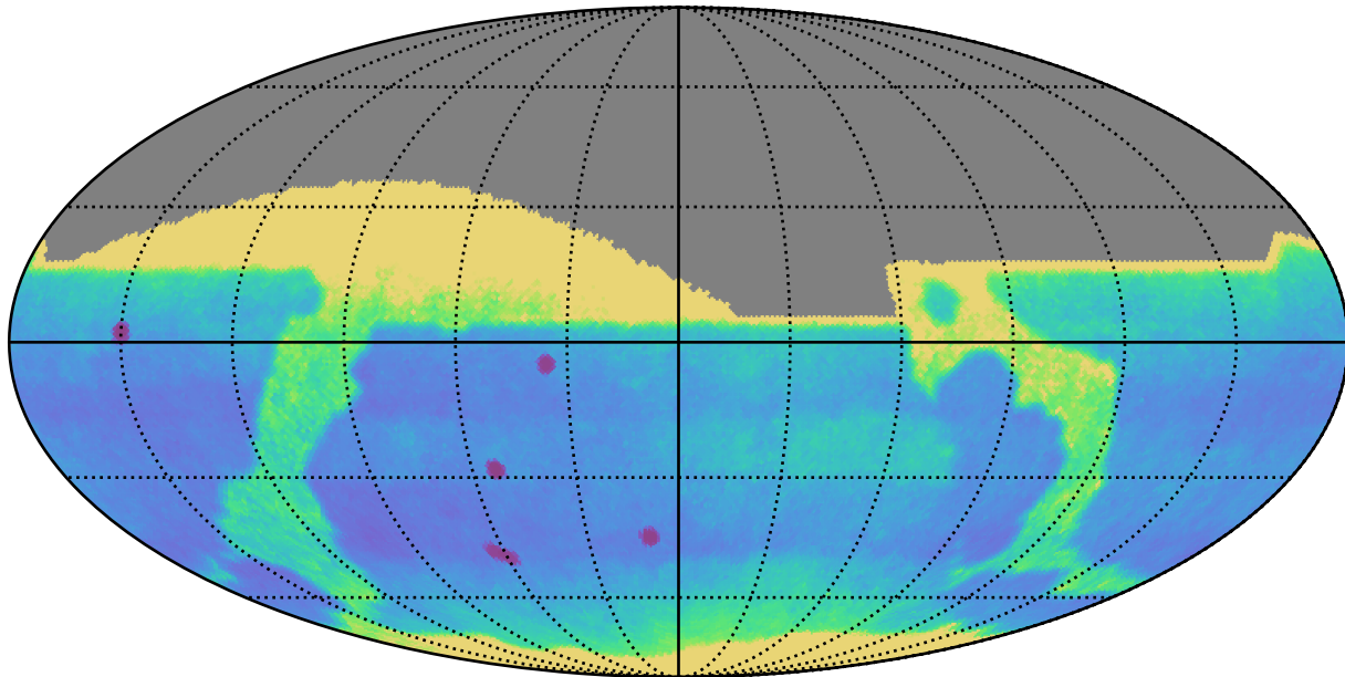
too_elab_r32_d2_gz_v3.4_10yrs : Proper Motion Uncert @ 24.0
