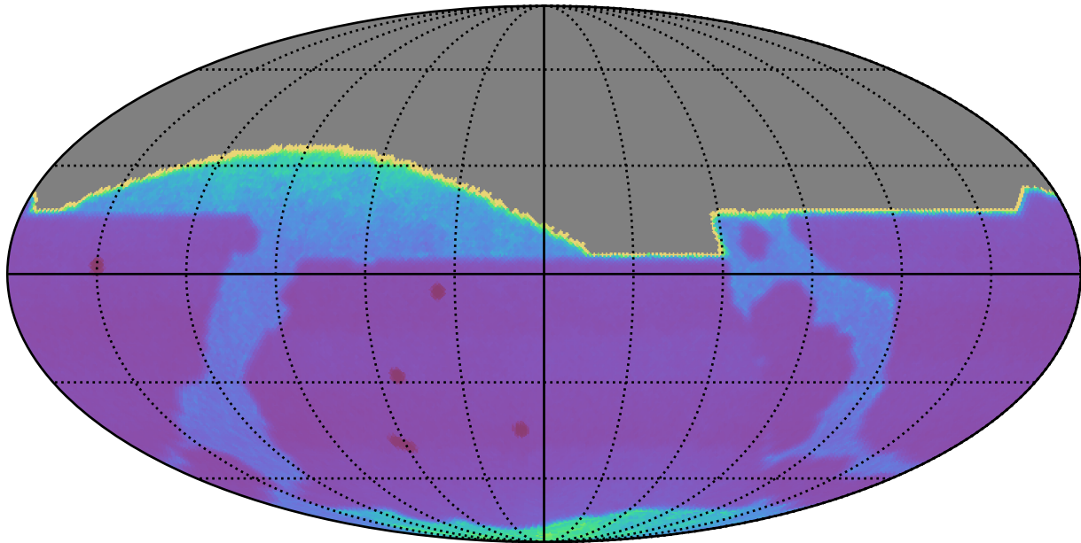
too_elab_r32_d2_gz_v3.4_10yrs : Proper Motion Uncert @ 20.5
