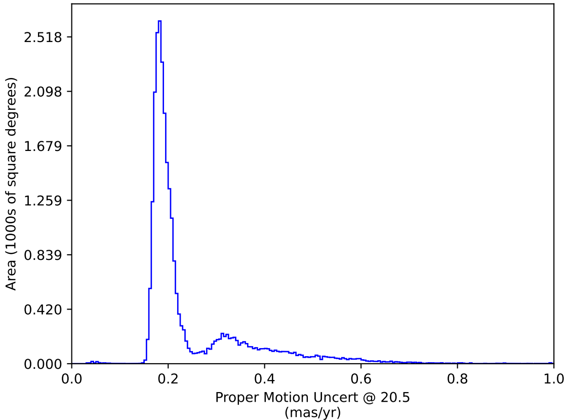
too_elab_r32_d2_gz_v3.4_10yrs : Proper Motion Uncert @ 20.5
