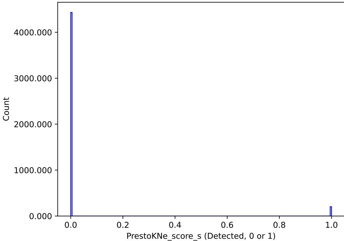
too_elab_r32_d2_gz_v3.4_10yrs : PrestoKNe_score_s
