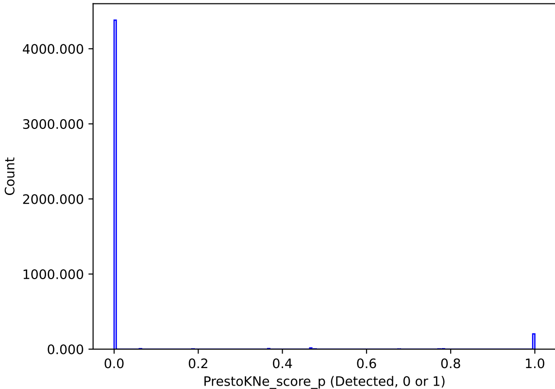
too_elab_r32_d2_gz_v3.4_10yrs : PrestoKNe_score_p
