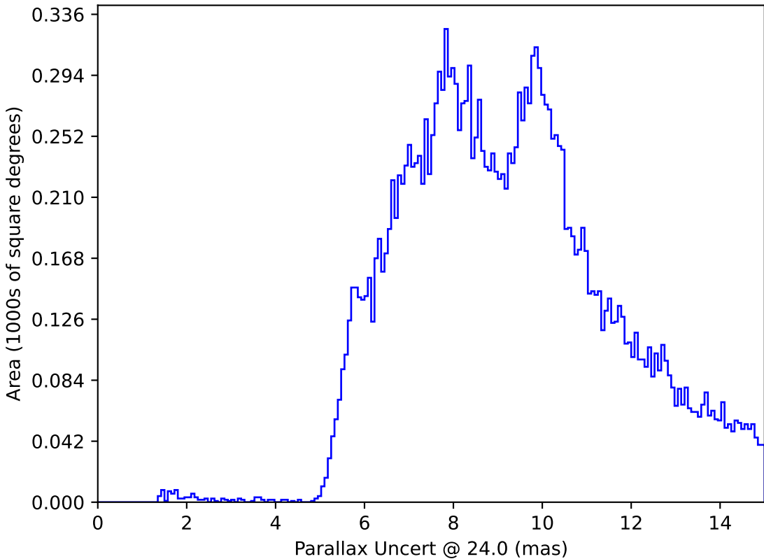
too_elab_r32_d2_gz_v3.4_10yrs : Parallax Uncert @ 24.0
