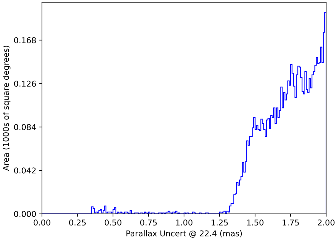
too_elab_r32_d2_gz_v3.4_10yrs : Parallax Uncert @ 22.4
