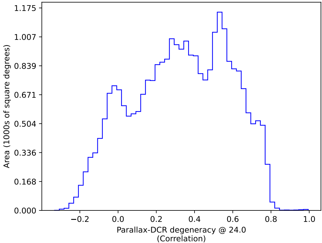
too_elab_r32_d2_gz_v3.4_10yrs : Parallax-DCR degeneracy @ 24.0
