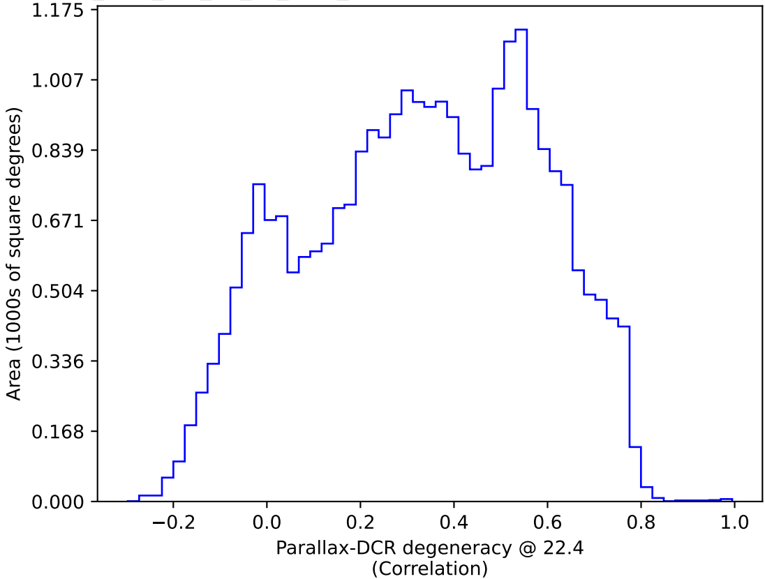
too_elab_r32_d2_gz_v3.4_10yrs : Parallax-DCR degeneracy @ 22.4
