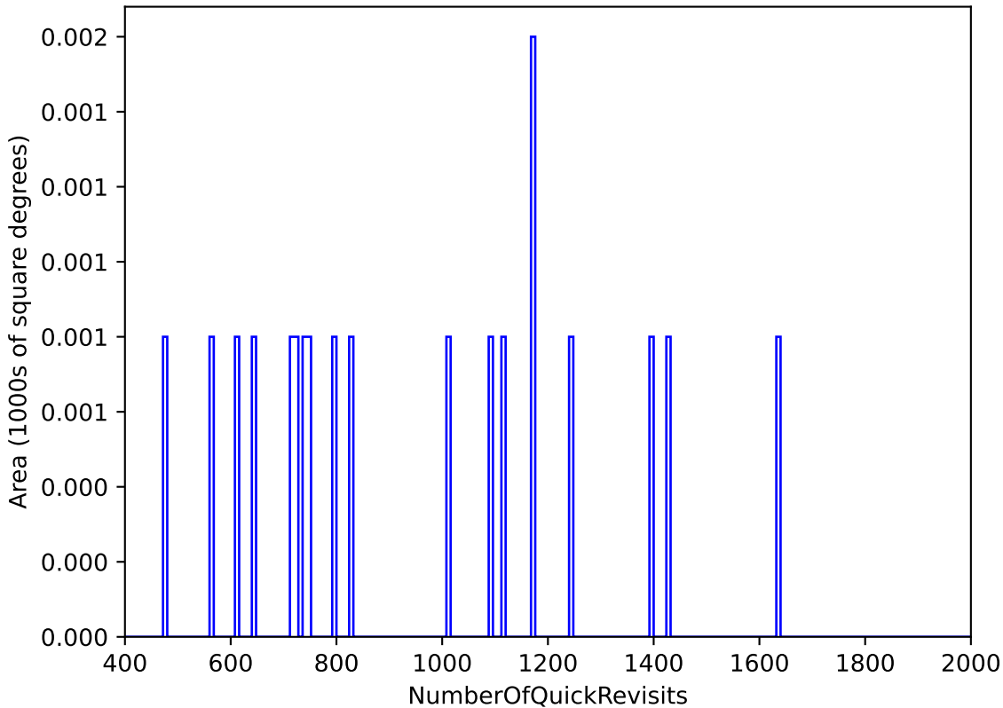
too_elab_r32_d2_gz_v3.4_10yrs : NumberOfQuickRevisits
