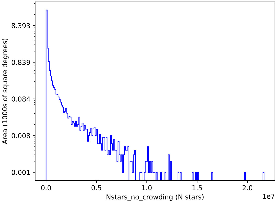
too_elab_r32_d2_gz_v3.4_10yrs r: Nstars_no_crowding
