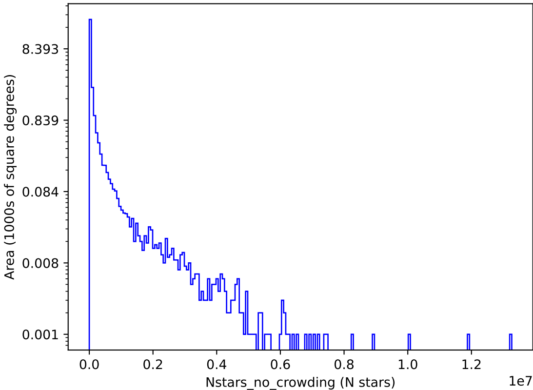
too_elab_r32_d2_gz_v3.4_10yrs g: Nstars_no_crowding
