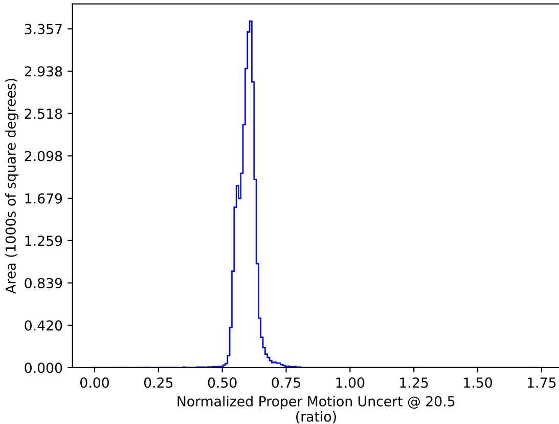
too_elab_r32_d2_gz_v3.4_10yrs : Normalized Proper Motion Uncert @ 20.5
