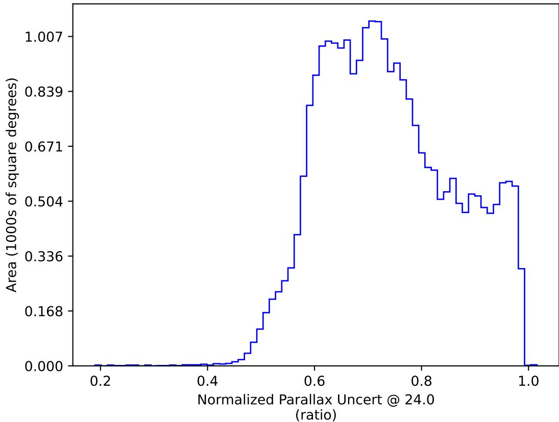
too_elab_r32_d2_gz_v3.4_10yrs : Normalized Parallax Uncert @ 24.0
