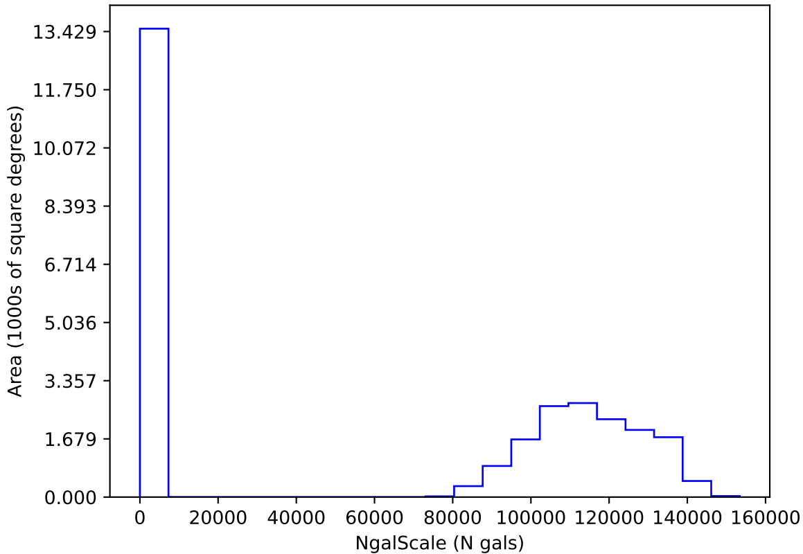
too_elab_r32_d2_gz_v3.4_10yrs i: NgalScale
