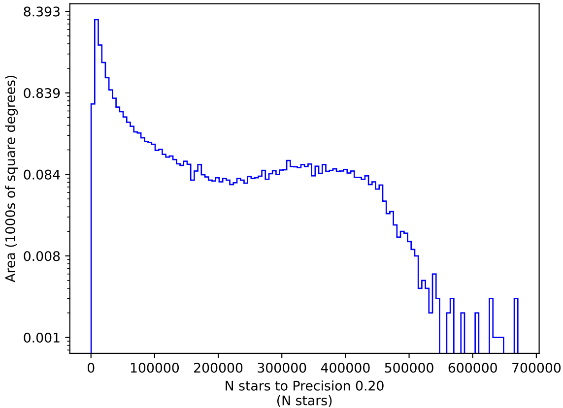
too_elab_r32_d2_gz_v3.4_10yrs y: N stars to Precision 0.20
