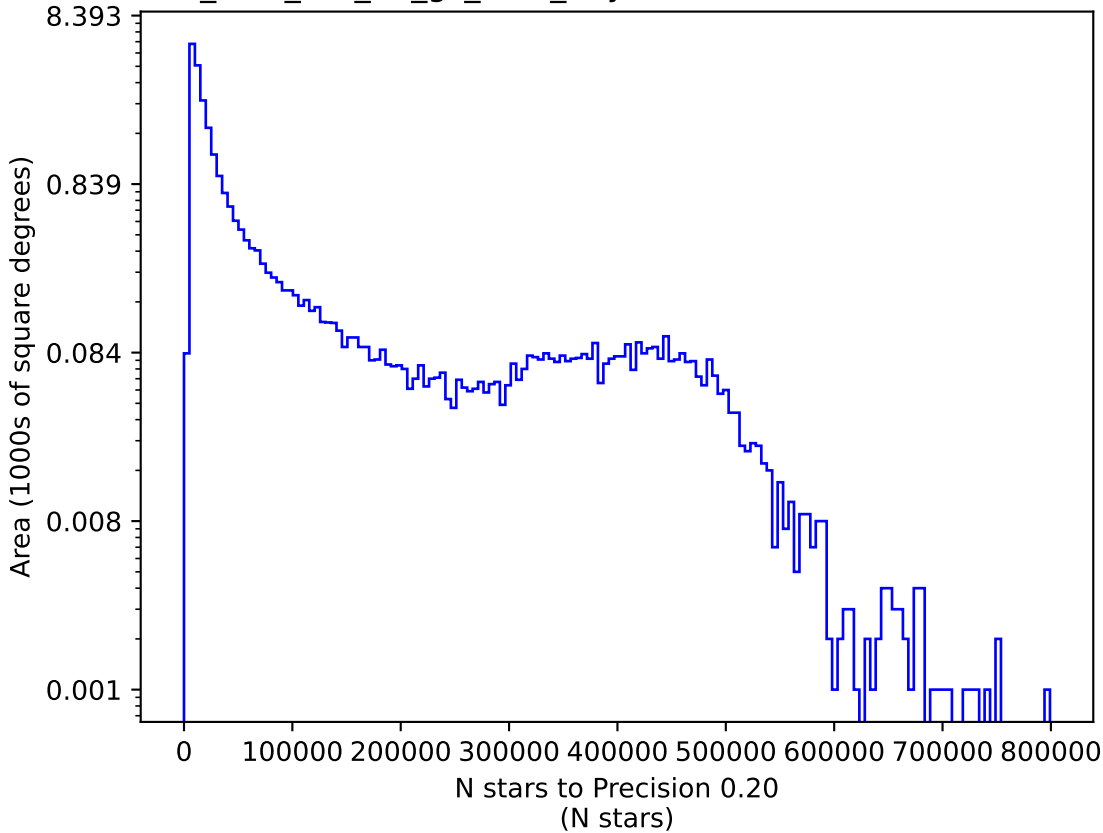
too_elab_r32_d2_gz_v3.4_10yrs i: N stars to Precision 0.20
