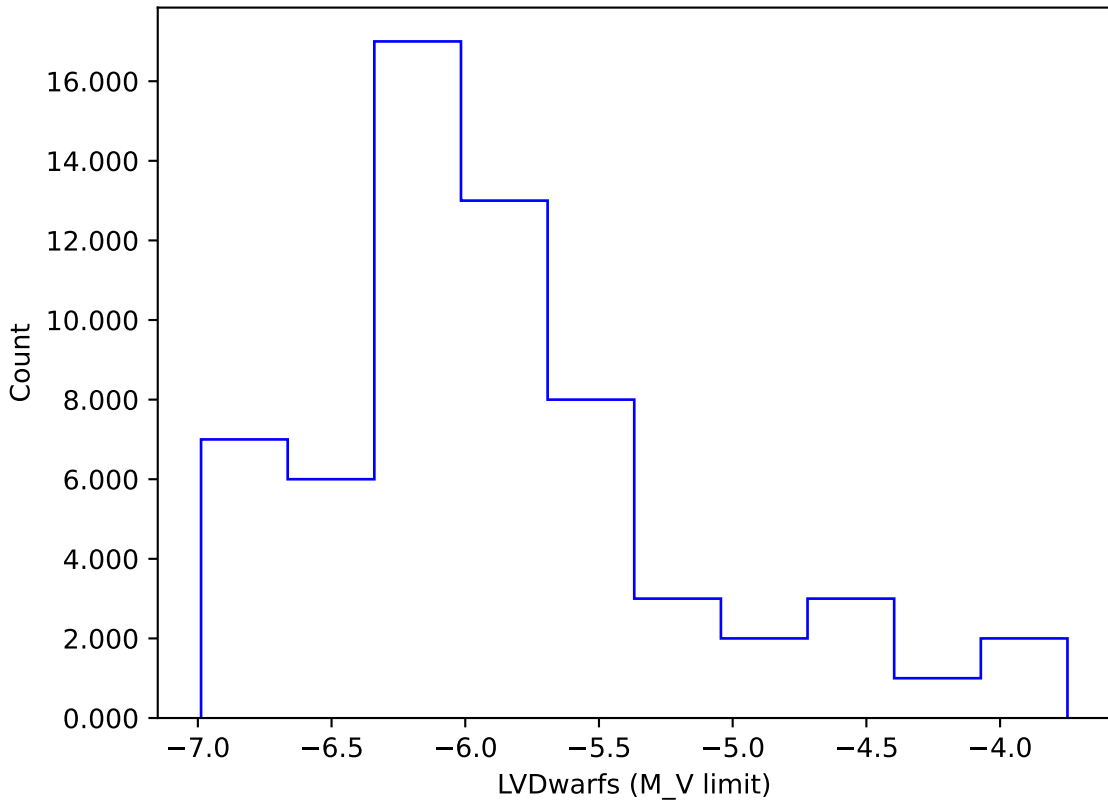
too_elab_r32_d2_gz_v3.4_10yrs gi: LVDwarfs
