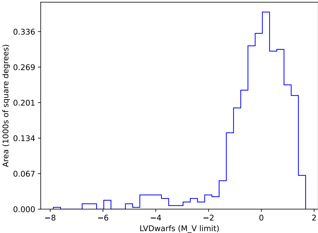
too_elab_r32_d2_gz_v3.4_10yrs gi SCP: LVDwarfs
