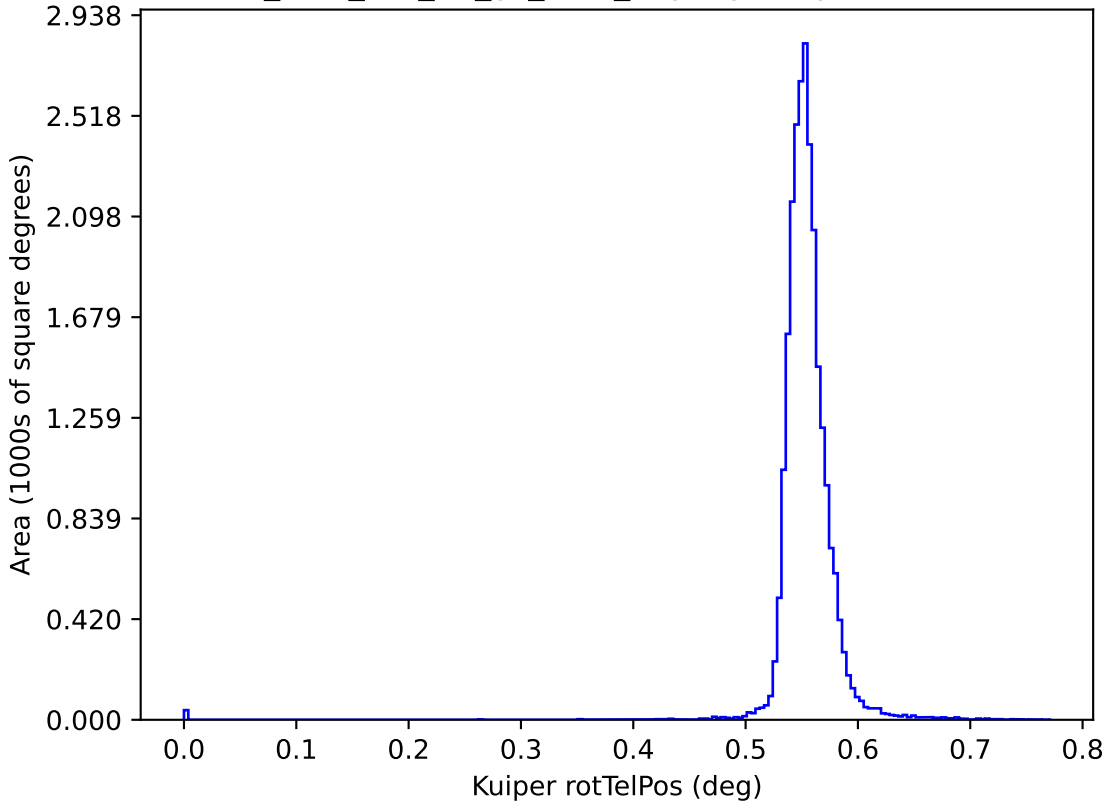
too_elab_r32_d2_gz_v3.4_10yrs y: Kuiper rotTelPos
