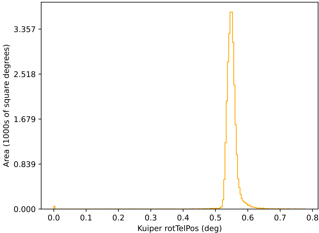
too_elab_r32_d2_gz_v3.4_10yrs r: Kuiper rotTelPos
