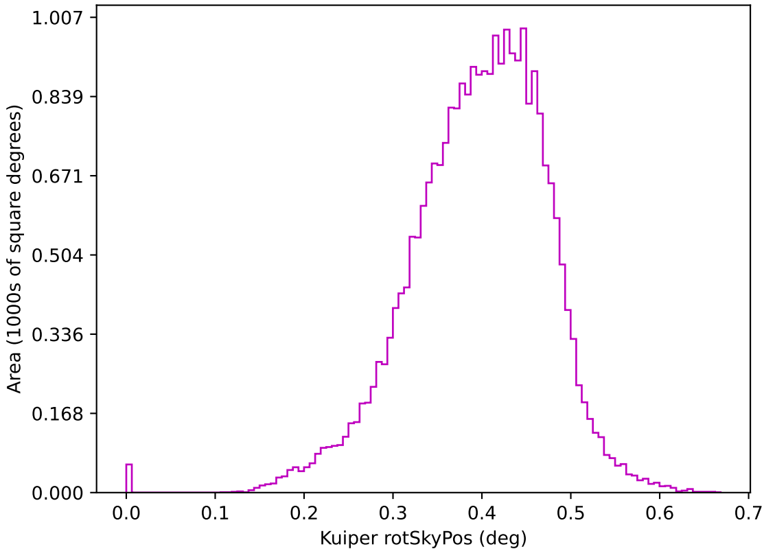
too_elab_r32_d2_gz_v3.4_10yrs z: Kuiper rotSkyPos
