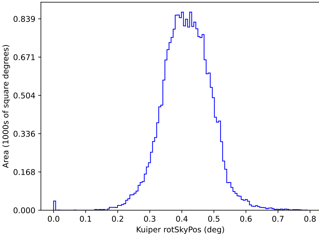
too_elab_r32_d2_gz_v3.4_10yrs y: Kuiper rotSkyPos
