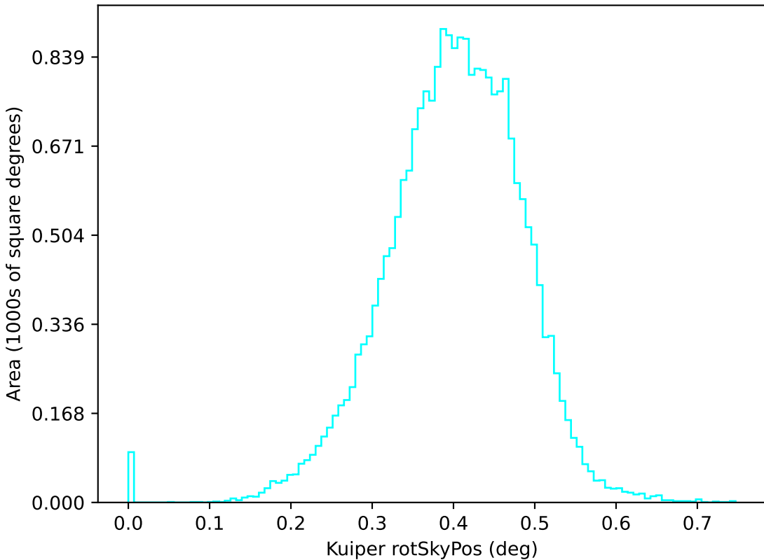
too_elab_r32_d2_gz_v3.4_10yrs u: Kuiper rotSkyPos
