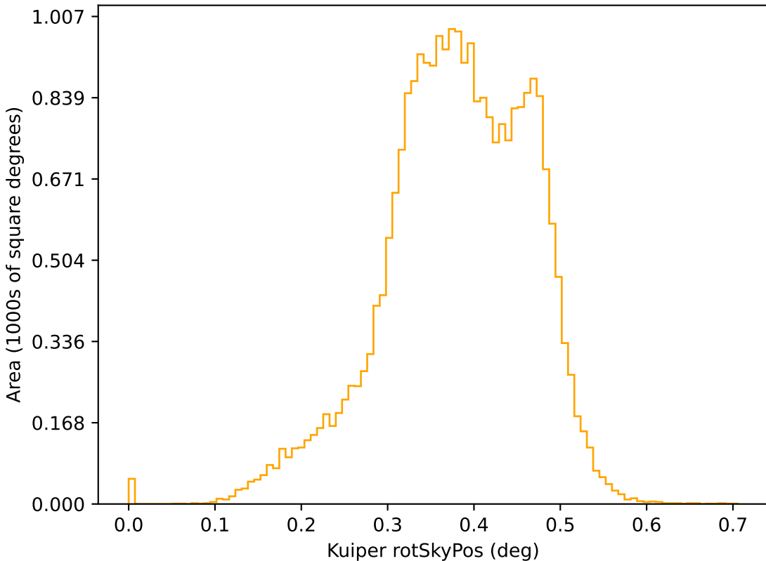
too_elab_r32_d2_gz_v3.4_10yrs r: Kuiper rotSkyPos
