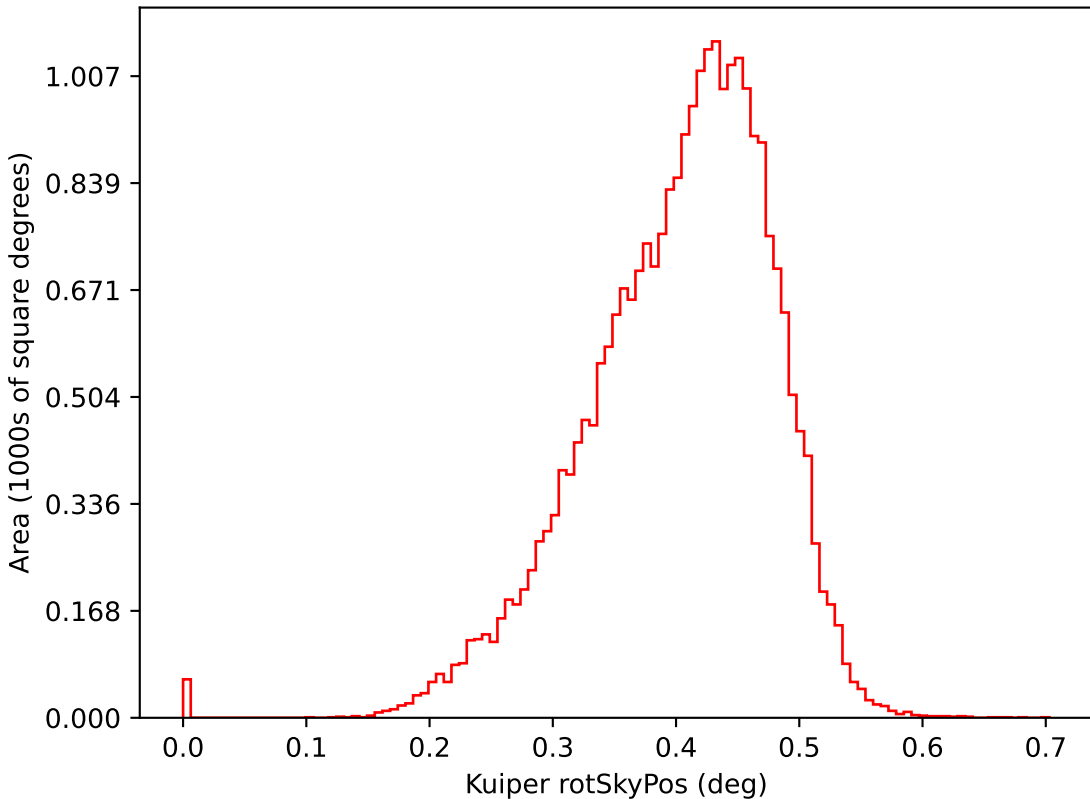
too_elab_r32_d2_gz_v3.4_10yrs i: Kuiper rotSkyPos
